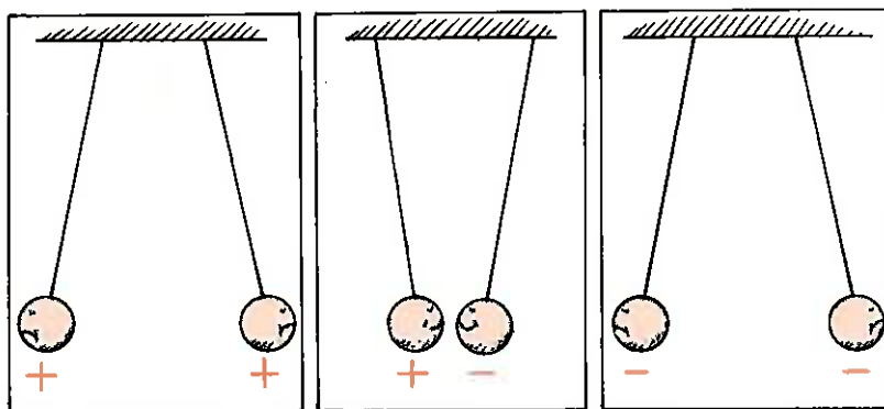
Fig. 32-3 Likes repel and opposites attract.
