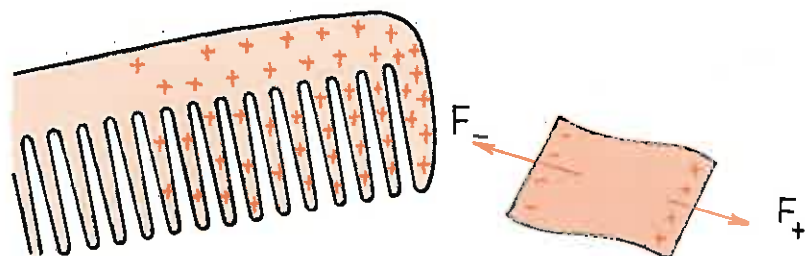
Fig. 32-12 A charged comb attracts an uncharged piece of paper because the force of attraction for the closer charge is greater than the force of repulsion for the farther charge. Closeness wins, and there is a net attraction.
