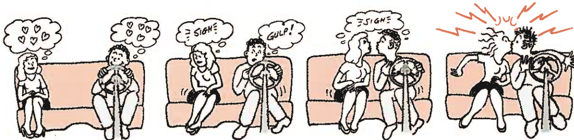
Fig. 32-7 Charging by friction and then by contact while parked at a drive-in movie.
