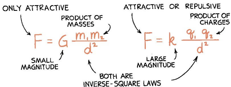
Fig. 32-5 Comparison of Newton's law of gravitation and Coulomb's law.
