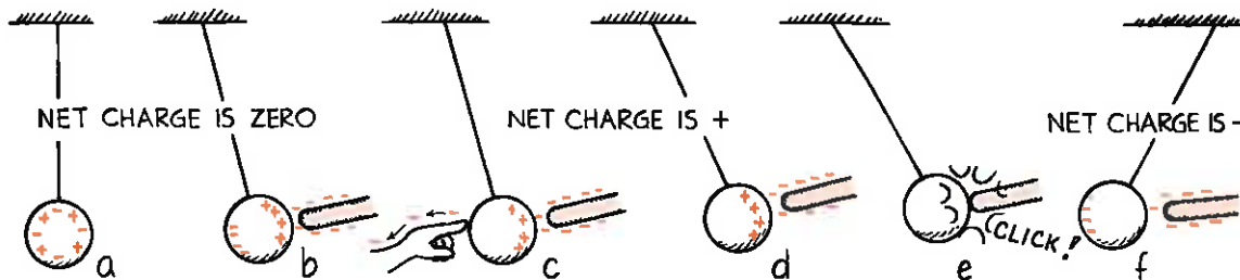
Fig. 32-9 Charge induction by grounding.
